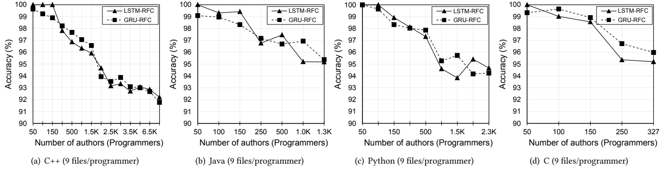
Figure 5: Accuracy of authorship identification of programmers with nine sample code files per programmer in four programming languages (C++, Java, Python, and C). Notice that the accuracy is always higher than 92% even with the worst of the two options of classifiers, and decay in the accuracy is insignificant despite a significant increase in the number of programmers.
